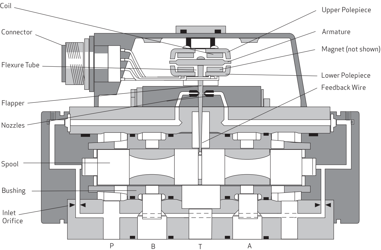
Electro-hydraulic Servo Valve Cut-away
