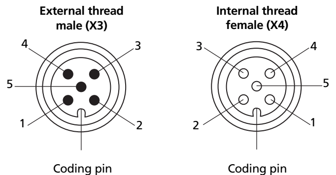
View on connection side of CANopen receptacle
