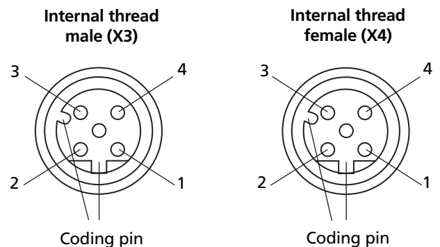
View on connection side of ETHERCAT receptacle
