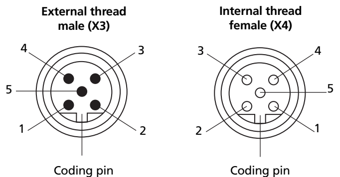
View on connection side of PROFIBUS-DP receptacle
