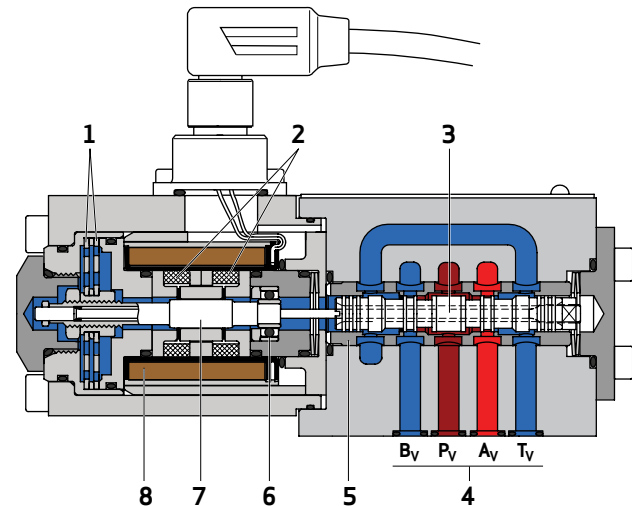
D633 Pilot Valve
